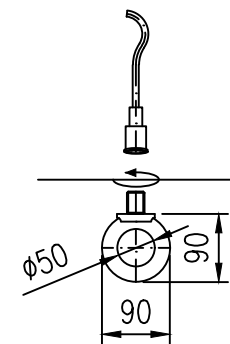
DETAIL MONT. OKA (1:10)
